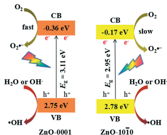
Fig. 7 Scheme of the band structures of ZnO-0001 and ZnO-10 \bar{1}\bar{0} , in which the conduction band (CB) positions determine the thermodynamic driving force for surface O_2 reduction reactions.
