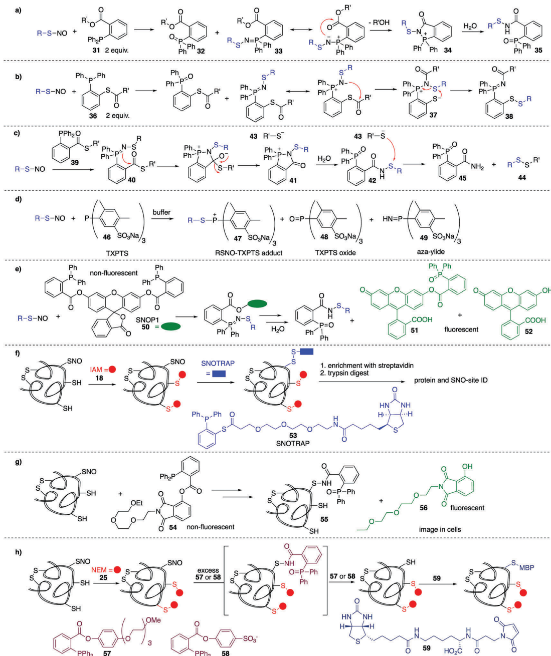
Fig. 7 (a and b) Reductive ligation of triarylphosphine derivatives with small molecule S -nitrosothiols. (c) Reductive ligation of triarylphosphine derivatives with S -nitrosothiols, followed by in situ conversion to an isolable disulfide. (d) Water soluble phosphine tris(4,6-dimethyl-3-sulfonatophenyl) phosphine trisodium salt (TXPTS) reacts with nitrosylated thiols. (e) Reductive ligation of triarylphosphine derivatives and nitrosylated thiols that generates a fluorescent product. (f) Reductive ligation of triarylphosphine derivatives with nitrosylated cysteines, leading to biotinylation at the key cysteine. (g) Cell-compatible reductive ligation of triarylphosphine derivatives and nitrosylated thiols that generates a fluorescent product. (h) A variation of the biotin switch method in which nitrosylated cysteines are selectively reduced with a phosphine-based reagent.
