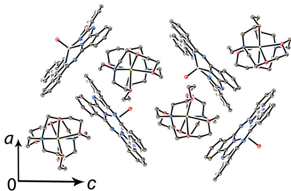
Fig. 6 View of the crystal structure of (\text{cryptand}(\text{Na}^+)\{\text{V}^{\text{IV}}\text{O}(\text{Pc}^{3-})\}^- \cdot \text{C}_6\text{H}_4\text{Cl}_2 (15) along the b axis and channels occupied by solvent \text{C}_6\text{H}_4\text{Cl}_2 molecules (not shown for clarity) and the cryptand( \text{Na}^+ ) cations. 27
