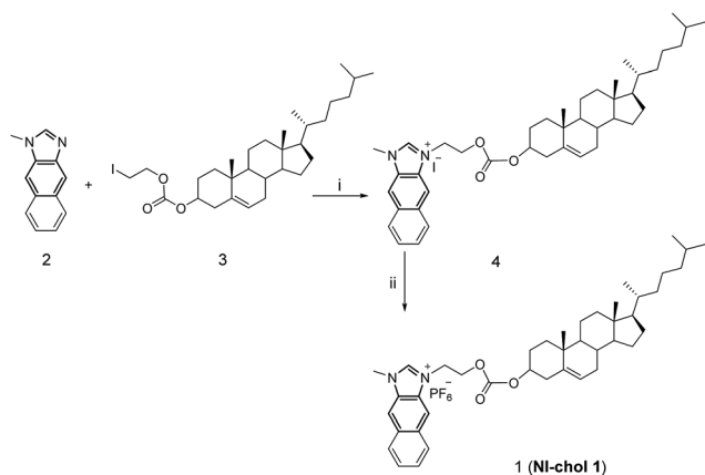
Scheme 1 The synthetic procedure of NI-chol 1 . (i) Acetonitrile, N 2 , reflux, 24 h, 81.1%; (ii) DMF, KPF 6 , 98.6%.
