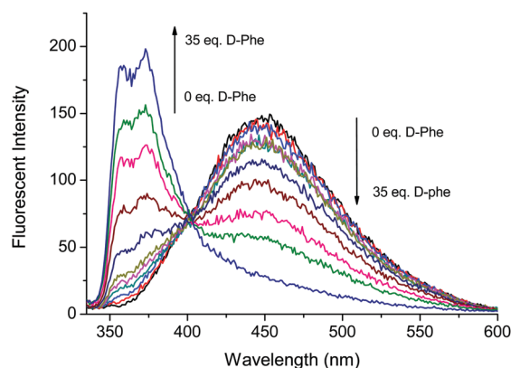
Fig. 3 Fluorescence based titrations of NI-chol 1 (10 μM) in CH 3 CN–DMSO (95:5, v/v) with various equivalents of Boc-D-Phe.
