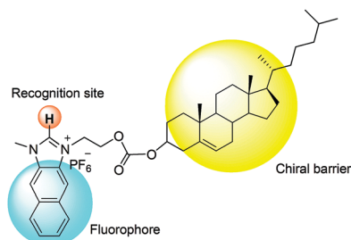
Fig. 1 Design strategy of NI-chol 1 .
