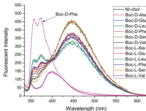
Fig. 2 Fluorescence changes of NI-chol 1 (10 μM) in CH 3 CN–DMSO (95:5, v/v) with D and L isomers of Ala, Glu, Leu, Phe, Ser and Val (500 μM). ( \lambda_{\text{ex}} = 325 nm, slit 3 × 5).
