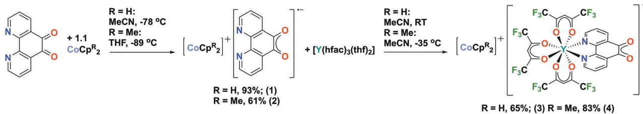
Scheme 2 Synthetic route to radical anion containing rare-earth transition metal complexes.
