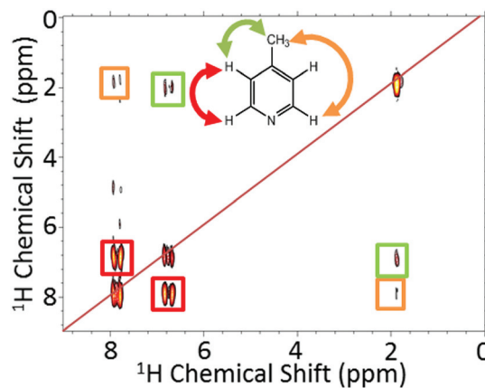
Fig. 6 2D gradient selective COSY coupled with SABRE for 52 mM 4-methylpyridine and 5.2 mM catalyst in methanol- d 4 . The COSY measurements used 64 increments over a bandwidth of 500 Hz (11.5 ppm), with single scan transients and re-hyperpolarization between each point. The total experiment time was around 36.4 minutes.
