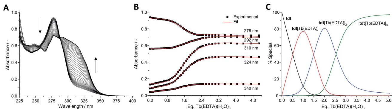
Fig. 3 (A) Absorption spectra, (B) experimental binding isotherms and corresponding fits (—), (C) speciation–distribution diagram for the UV-visible titration of tdt (12 \mu\text{M} ) with \text{Tb}(\text{EDTA})\cdot(\text{H}_2\text{O})_3 in methanol at 298 K.
