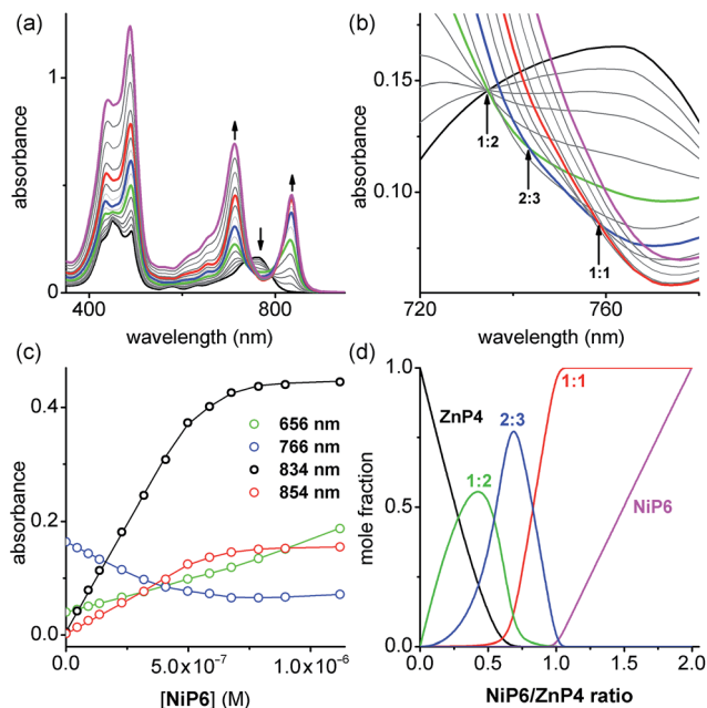
Fig. 6 (a) UV-vis-NIR titration of ZnP4 ( [ZnP4] = 0.73 \mu\text{M} ) with NiP6 in dry \text{CH}_2\text{Cl}_2 at 298 K. Arrows indicate increasing or decreasing absorption (black, free ZnP4; green, 1 : 2 complex; blue, 2 : 3 complex, red, 1 : 1 complex and magenta, the end spectrum of NiP6-saturated-ZnP4). (b) Zoom-in of the change of isosbestic points in the absorption spectra. Arrows point out three subsequent isosbestic points at 0.5, 0.7 and 1.0 equivalents of NiP6, which is consistent with NiP6 : ZnP4 complexes of 1 : 2, 2 : 3 and 1 : 1 stoichiometries, respectively. (c) Binding isotherm (open dots) derived from absorption data at various wavelengths and fit obtained from global analysis with SPECFIT (solid lines). (d) The speciation plots as a function of the ratio [NiP6]/[ZnP4] (black, free ZnP4; green, 1 : 1 complex; blue, 2 : 3 complex, red, 1 : 1 complex and magenta, free NiP6).
