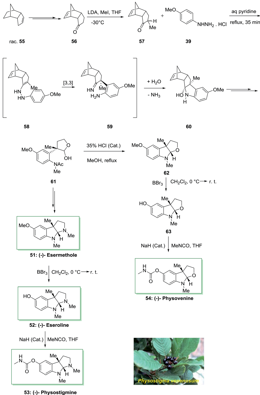
Scheme 9 Total synthesis of (–)-esermethole 51 , (–)-eseroline 52 , (–)-physostigmine 53 and (–)-physovine 54 .
