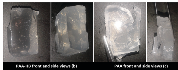
Fig. 12 (a) Change in the SR10/SR2 ratio during three cycles of dynamic swelling revealed higher pH sensitivity of PAA-HB hydrogels compared to that of PAA samples. After 3 cycles, the better dimensional stability of (b) PAA-HB samples compared to that of (c) PAA samples was in general agreement with the enhanced mechanical properties from HB.
