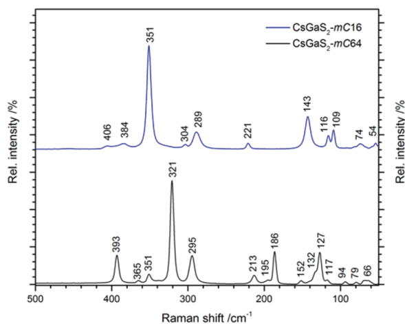
Fig. 8 Raman spectra of the \text{CsGaS}_2 polymorphs (black line: mC64 , blue line: mC16 ).
