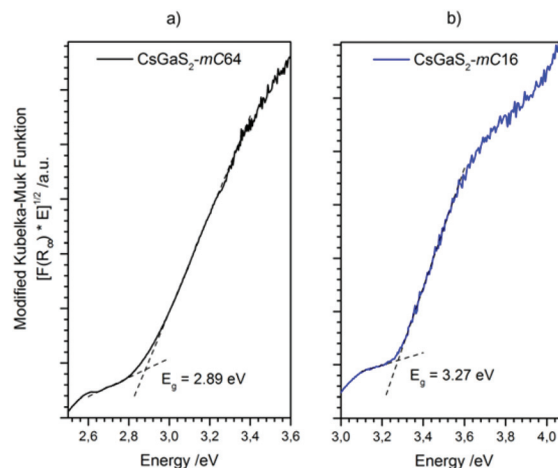
Fig. 9 Diffuse reflectance spectrum of (a) \text{CsGaS}_2\text{-}mC64 and (b) \text{CsGaS}_2\text{-}mC16 . Optical band gaps were determined by extrapolation of the linear part of the modified Kubelka–Munk function onto the baseline, as indicated by the dashed lines.
