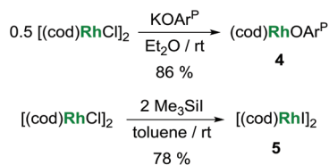
Scheme 3 Alternative syntheses for (\text{cod})\text{Rh}(\text{OAr}^{\text{P}}) (4) and [(\text{cod})\text{RhI}]_2 (5).
