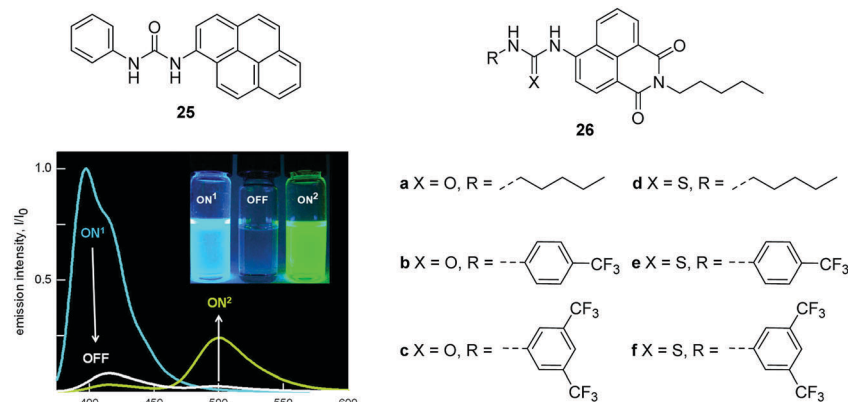
Fig. 12 Structures of 25 , 26a-f and the emission spectra taken upon addition of F^- to 25 (0.01 mM) in MeCN. Reproduced from ref. 25 with the permission of the American Chemical Society.
