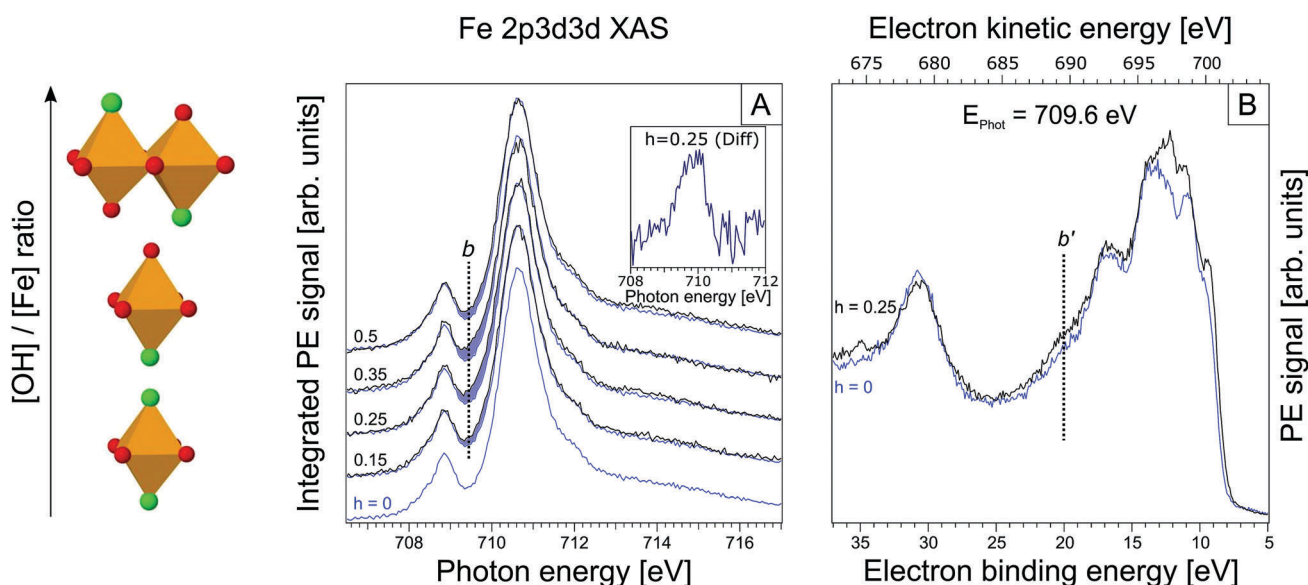
Fig. 3 (A) Partial electron yield X-ray absorption spectra at the iron 2p_{3/2} . The h = 0 XA spectrum is reproduced in each tier for h \neq 0 . Again, spectral differences are highlighted in blue. The inset displays the actual differential spectrum for h = 0.25 ; b is the maximum of this absorption band. (B) RPE spectrum for h = 0.25 solution, measured at 709.6 eV excitation photon energy (maximum of the main absorption band in Fig. 3A). In blue the RPE spectrum for h = 0 is shown.
