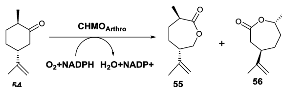
Scheme 18 CHMO-Arthro catalyzed Baeyer–Villiger oxidation of (+)- trans -dihydrocarvone ( 54 ) with formation of the formal “abnormal” product 55 generated by the WT enzyme and normal product 56 provided by an evolved mutant thereof. 75
