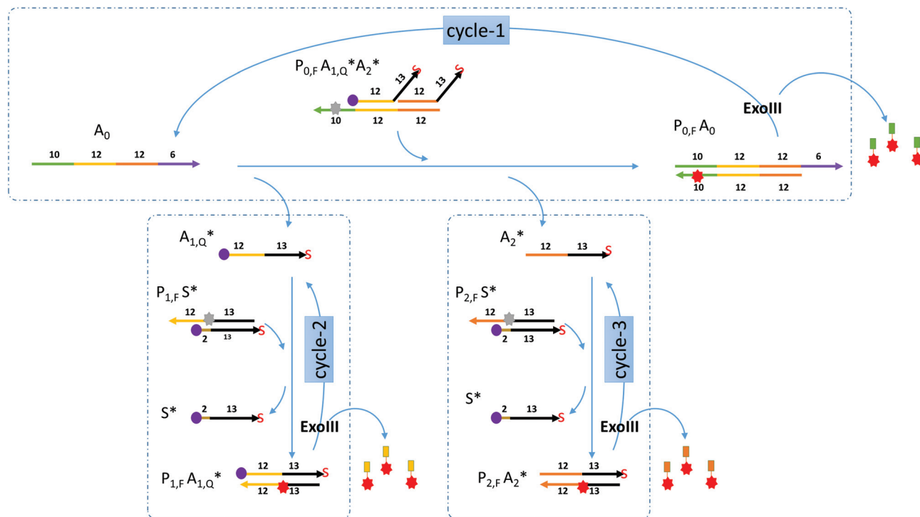
Fig. 1 Schematics of the nucleic acid circuitry. The target analyte ( A_0 ) binds to P_0 and releases A_1 and A_2 and gives off a fluorescent signal. Exo III then digests Q_0 at the 3' blunt end for target recycling. At the same time A_1 and A_2 bind to their respective probes P_1 and P_2 to form Q_1 and Q_2 which also similarly give off a fluorescent signal and are digested by exo III for two more cycles of target recycling. These three iterative cycles produce a fluorescent signal whenever Q probes are formed. (similar colors represent complementary sequences with the arrowhead signifying the 3' end. The arrowhead with "S" means that the 3' end is modified with a phosphorothioate linkage. The numbers correspond to the length of the segment below or above.)
