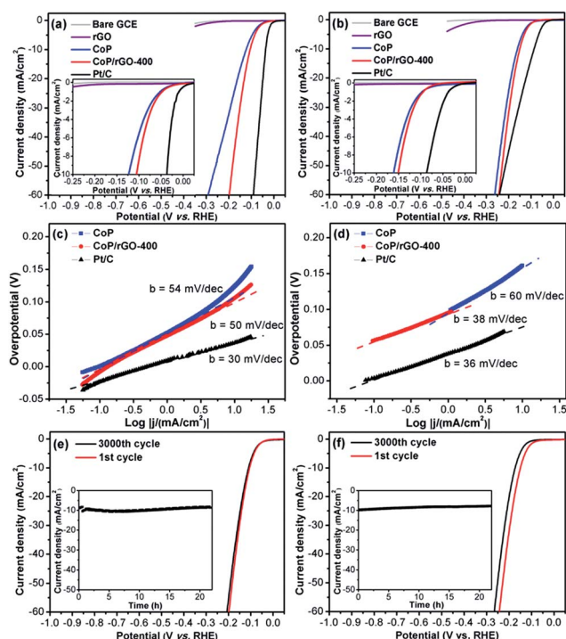
Fig. 2 Electrochemical HER activity of CoP/rGO-400. (a) LSV curves, (c) Tafel slopes and (e) durability test in 0.5 M \text{H}_2\text{SO}_4 solution; (b) LSV curves, (d) Tafel slopes and (f) durability test in 1 M KOH solution. Insets in (e) and (f): time-dependent current density curves under static overpotentials of 105 mV in 0.5 M \text{H}_2\text{SO}_4 and 150 mV in 1 M KOH solution, respectively.
