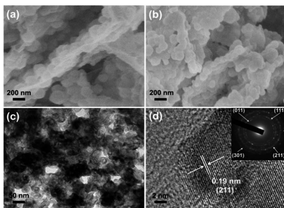
Fig. 1 Scanning electron microscope (SEM) images of (a) ZIF-67/GO and (b) CoP/rGO-400. (c) Transmission electron microscopy (TEM) and (d) high-resolution TEM images of CoP/rGO-400 (inset in (d): SAED pattern for CoP nanocrystal).
