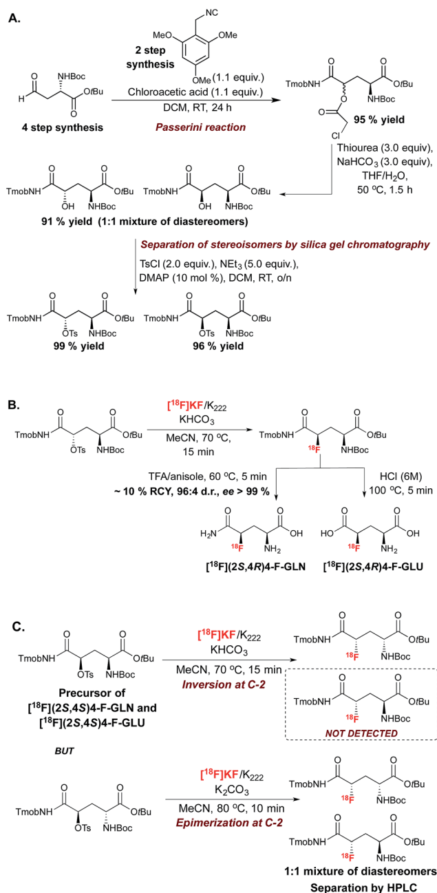
Scheme 2 (A.) Synthesis of the substrates for the radiosynthesis of ^{18}\text{F} ]-4-F-GLU and ^{18}\text{F} ]-4-F-GLN. (B.) Radiosynthesis of ^{18}\text{F} -(2 S ,4 R )-4-F-GLU and ^{18}\text{F} -(2 S ,4 R )-4-F-GLN. (C.) Radiosynthesis of ^{18}\text{F} -(2 S ,4 S )-4-F-GLU and ^{18}\text{F} -(2 S ,4 S )-4-F-GLN precursors. Tmob = 2,4,6-trimethoxybenzyl.
