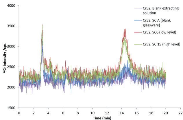
Fig. 6 HPLC-ICP-MS chromatogram of Cr species in mainstream smoke from cigarette spiked two different spike levels ( 5.80 and 9.80 \mu g g^{-1} of chromium, respectively) using 2.8 mM TPABr and 4 mM EDTA (pH 8.5) as extractant. 0.18 mM, 1 mM EDTA (pH 8) as mobile phase at a flow rate of 0.8 mL min^{-1} .
