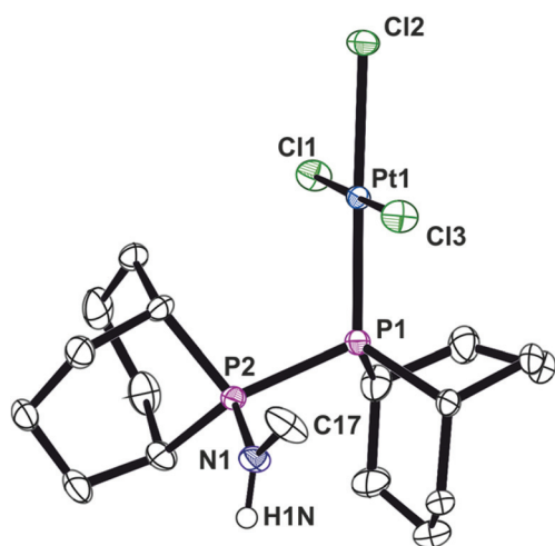
Fig. 5 Crystal structure of [\text{PtCl}_3(\text{L}'_e)\cdot\text{HCl}] ( 5 ). All hydrogen (except H1N) atoms, a \text{CH}_2\text{Cl}_2 molecule (50% occupied) and one \text{C}_2\text{H}_2\text{Cl}_4 molecule have been omitted for clarity. Selected bond lengths (Å) and angles (°); Pt(1)–P(1) 2.2194(13), Pt(1)–Cl(1) 2.3085(12), Pt(1)–Cl(2) 2.3683(12), Pt(1)–Cl(3) 2.2988(12), P(1)–P(2) 2.2797(19), P(2)–N(1) 1.629(4), N(1)–C(17) 1.468(7), N(1)–H(1N) 0.8800, P(1)–Pt(1)–Cl(3) 88.86(5), P(1)–Pt(1)–Cl(1) 92.80(5), Cl(3)–Pt(1)–Cl(1) 177.36(5), P(1)–Pt(1)–Cl(2) 177.89(5), Cl(3)–Pt(1)–Cl(2) 89.39(5), Cl(1)–Pt(1)–Cl(2) 88.99(5), Pt(1)–P(1)–P(2) 108.26(6), N(1)–P(2)–P(1) 111.95(19).
