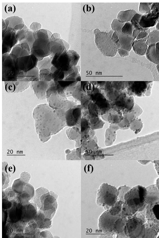
Fig. 3 TEM images of (a) 4% Ru–1% Pd/TiO 2 ; (b) 3% Ru–2% Pd/TiO 2 ; (c) 2.5% Ru–2.5% Pd/TiO 2 ; (d) 2% Ru–3% Pd/TiO 2 ; (e) 1% Ru–4% Pd/TiO 2 and (f) 0.5% Ru–4.5% Pd/TiO 2 .
