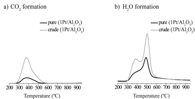
Fig. 5 a) CO 2 and b) H 2 O formation during thermogravimetric analyses of a spent 1Pt/Al 2 O 3 catalyst after the APR of pure (black) and crude (gray) glycerol.
