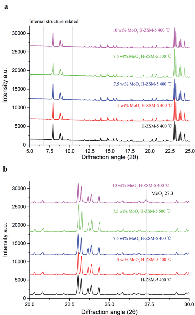
Fig. 2 (a) X-ray diffraction patterns (2θ = 5–25°) of MoO 3 /ZSM-5 samples with various MoO 3 loadings and prepared at 400 °C/500 °C. (b) X-ray diffraction patterns (2θ = 20–30°) of MoO 3 /ZSM-5 samples with various MoO 3 loadings and prepared at 400 °C/500 °C.
