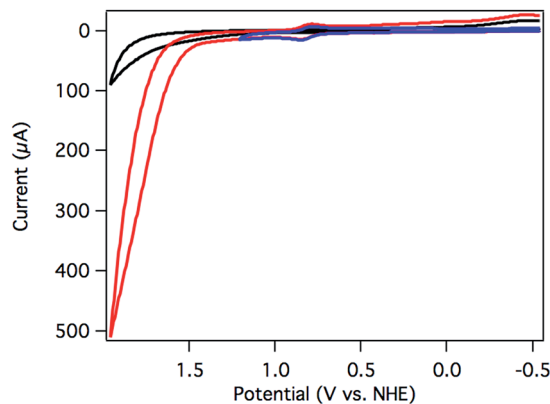
Fig. 3 CV of [Ru(Py 3 PO)(bpy)(OH 2 ) 2+ ] 2+ ( 3 ) swept anodically to 1.95 V (red) and 1.2 V (blue) vs. NHE. A catalyst-free background scan is shown in black. The reduction near -0.5 V is assigned to O 2 reduction. Conditions: 250 mV s -1 scan rate, pH 7 0.1 M phosphate buffer, 3 mm glassy carbon disk working electrode, Pt wire counter electrode, Ag/AgCl reference electrode.
