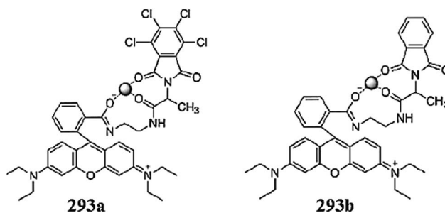
Fig. 257 Chemical structure of the ligand–Hg 2+ complexes.
