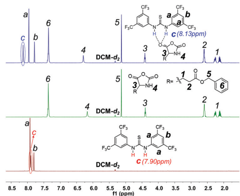
Fig. 2 Expanded ^1\text{H} NMR spectra of TU-S, Glu-NCA and TU-S/Glu-NCA (1 : 1) mixture (500 M, 25 ^\circ\text{C} , \text{CD}_2\text{Cl}_2 , for full spectra see Fig. S1 and S2 \dagger ).
