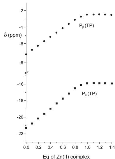
Fig. 3 Plot of the chemical shifts of the terminal (P β ) and central (P α ) phosphorous nuclei of TP in the presence of an increasing amount of the Zn(II) complex of 1 at 162 MHz, pH 7 and 308 K.
