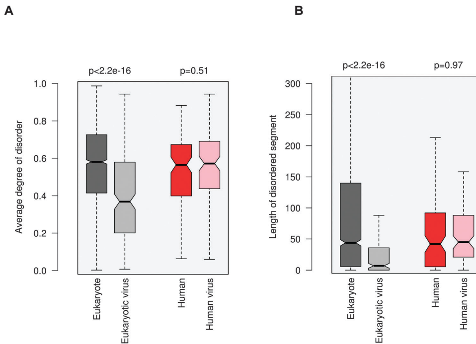
Fig. 3 Disorder properties of the protein regions flanking the eukaryotic (dark gray), eukaryotic virus (light gray), human (dark red) and human virus (light red) ELMs. The human and human virus ELMs target common host motif-binding domains. (A) The average degree of disorder of the 20AA flanking region. (B) The length of the disordered segment flanking the motif. The p values were computed using the Wilcoxon test.
