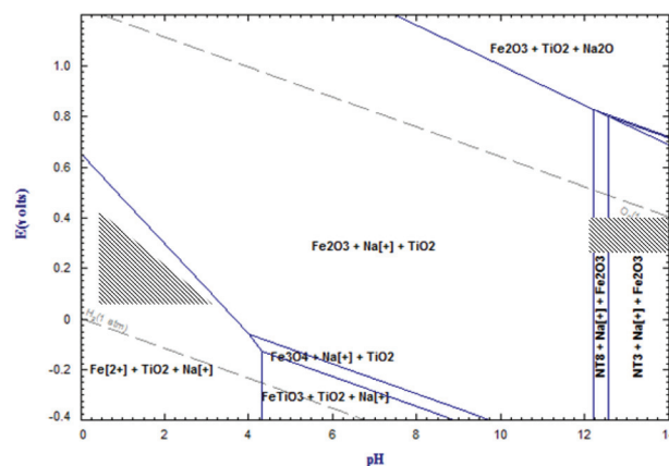
Fig. 16 The E_h -pH diagram of the system Na-Ti-Fe-O calculated by Fact-Sage 6.4 software at 70\text{ }^\circ\text{C} . NT3: Na_8Ti_5O_{14} , NT8: Na_8Ti_5O_{14} . 66
