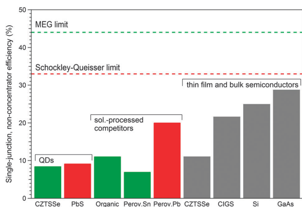
Fig. 6 Comparison of record power conversion efficiencies for PVs based on CZTSSe 177 and PbS QDs, 176 organics, perovskites (Pb-based 182 and Sn-based 183,184 ), and more established CZTSSe and CIGS thin films and Si and GaAs bulk semiconductors (unless otherwise referenced, data were taken from the NREL Research Cell Efficiency chart 185 ). Shockley–Queisser 186 and MEG 187 limits are shown using red and green dashed lines, respectively.
