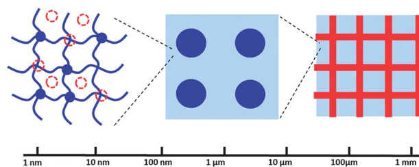
Fig. 9 A promising strategy to design next-generation tough hydrogels is to integrate multiple mechanisms across multiple length scales into a hydrogel. For example, a tough hydrogel may integrate fiber-reinforcement at the macro-/meso-scale, high-functionality crosslinkers at the micro-scale, and hybrid crosslinkers at the nano-scale.
