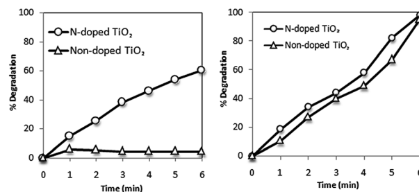
Fig. 4 Photocatalytic degradation of direct black 38 as a function of time under visible light (left) and sunlight (right). Experimental conditions: C_0 = 0.055 \text{ g L}^{-1} , C_{\text{catalyst}} = 1.0 \text{ g L}^{-1} , \text{pH} = 2.5 , T = 25^\circ \text{C} . 153
