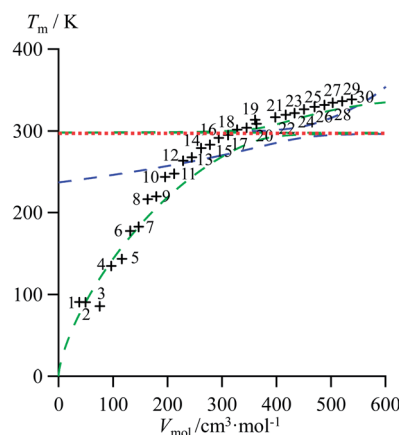
Fig. 8 Correlations between molar volumes V_{\text{mol}} and melting temperatures T_m for linear alkanes C_nH_{2n+2} ( n = 1-30 ) fitted using a parabolic H/S function (blue trace) or a reciprocal Hill plots (green trace). The horizontal dotted red trace corresponds to the asymptotic behaviour occurring when the melting temperature approaches the selected reference temperature T^0 = 298.15 \text{ K} .
