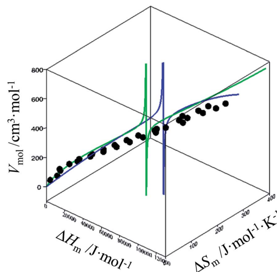
Fig. 7 Three-dimensional V_{\text{mol}} , \Delta H_m , \Delta S_m plot for linear alkanes fitted with a parabolic H/S function (blue trace) or a reciprocal Hill plots (green trace). An asymptotic behaviour is expected to occur when the melting temperature approaches the selected reference temperature T^0 = 298.15 \text{ K} .
