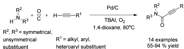
Scheme 42 Reagents and conditions: alk-1-yne (1 mmol), secondary amine (1.5 mmol), 10% Pd/C (8 mol%), CO/O 2 pressure (5/1 atm), TBAI (0.90 mmol), 1,4-dioxane (10 mL), temperature 80^\circ\text{C} , time 14 h.
