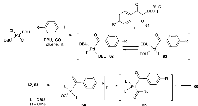
Scheme 77 Proposed mechanism for the double carbonylation reaction of aryl halides in the presence of DBU.
