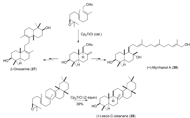
Scheme 40 Synthesis of myrrhanol A, (+)-seco-C-oleanane, and β-onocerine via \text{Cp}_2\text{TiCl} promoted epoxypolyene cyclisation.
