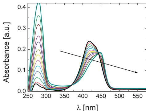
Fig. 4 Absorbance spectra of P1 solution in PBS ( 0.005 \text{ g L}^{-1} ) at 15^\circ\text{C} containing varying amounts of the antibody [from 6.7 \text{ nM} to 660 \text{ nM} ]. The direction of the arrow shows the increase in antibody concentration.
