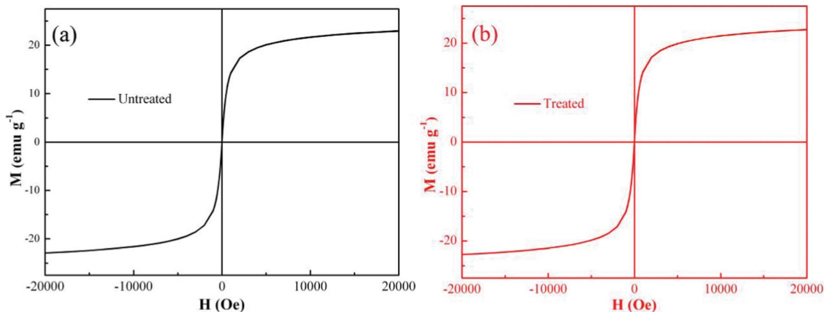
Fig. 8 Room-temperature magnetic hysteresis loops of (a) the synthesized PNCs, and (b) the PNCs after 5 min treatment with 20.0 mL Cr(VI) solution (pH = 1.0; 4.0 \text{ mg L}^{-1} ).
