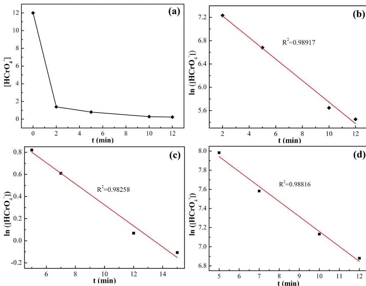
Fig. 7 (a) Cr(VI) concentration change of 10.0 mg PNCs after treatment with 20.0 mL Cr(VI) solution (pH = 1.0; 12.0 \text{ mg L}^{-1} ) with different treatment periods at room temperature; (b) corresponding kinetic plot in pH = 1.0 Cr(VI) solution; (c) kinetic plot after treatment with 20.0 mL Cr(VI) solution of pH = 7.0, 9.0 \text{ mg L}^{-1} and (d) pH = 11.0, 5.0 \text{ mg L}^{-1} at room temperature.
