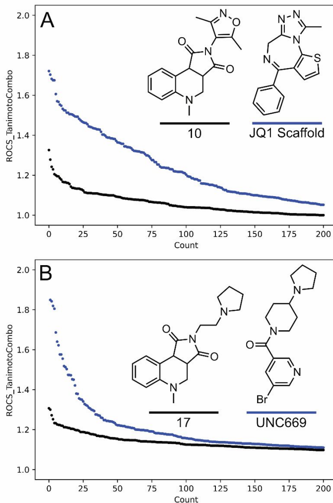
Figure 4. Analysis of the top 200 ROCS ranked BRD4 or L3MBTL1 ligands in the ChEMBL database compared with exemplar compounds bearing privileged epigenetic chemotypes. Count refers to the ROCS ranking where 1 is the best ranked compound (most similar). A: Compound 10 (black) or the scaffold of JQ1 (blue) vs. BRD4 ligands deposited to ChEMBL (2168 molecules). B: Compound 17 (black) or UNC669 (blue) vs. L3MBTL1 ligands deposited to ChEMBL (10,847 molecules, UNC669 was removed from the test set).
