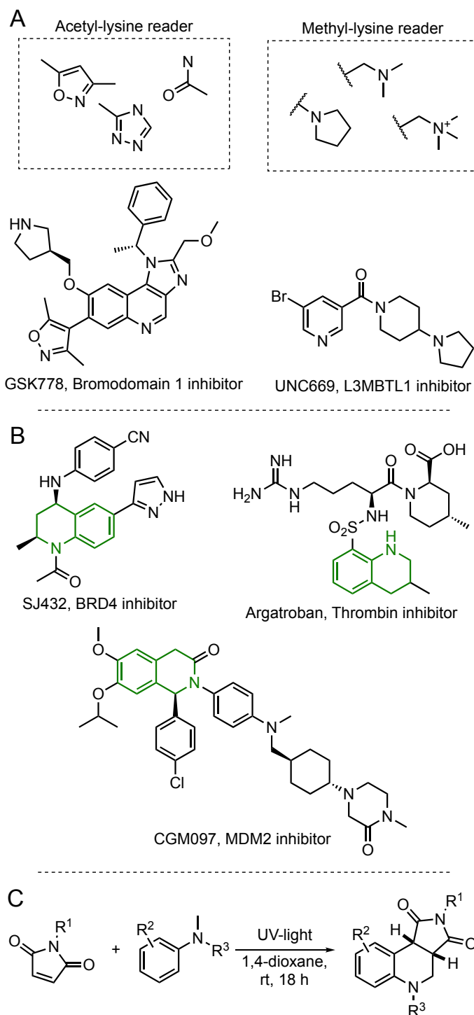
Figure 1. Exemplar epigenetic bioisosteres and ligands containing a tetrahydroquinoline pharmacophore highlighted in green. A: Examples of chemotypes employed as part of inhibitors of acetyl-lysine readers and
