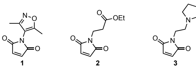
Figure 2. Maleimide building blocks used in the synthesis of the epigenetic focused tetrahydroquinoline library.
