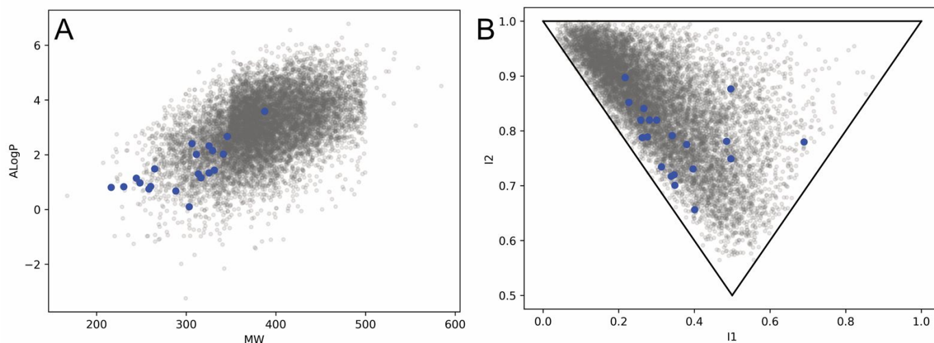
Figure 3. Comparison of molecular properties for this compound collection and a commercially available epigenetic compound collection. A: Molecular weight vs ALogP. B: Principal Moment of Inertia plot. The commercially available epigenetic library is shown in grey and our focused library described is shown in blue. ALogP and principal moment of inertia (PMI) were calculated in RDKit. PMI represents the three-dimensional shape of a molecule where rod-like molecules are in the top left, disc-like molecules are at the lower middle, and sphere-like molecules are in the top right of the plot.
