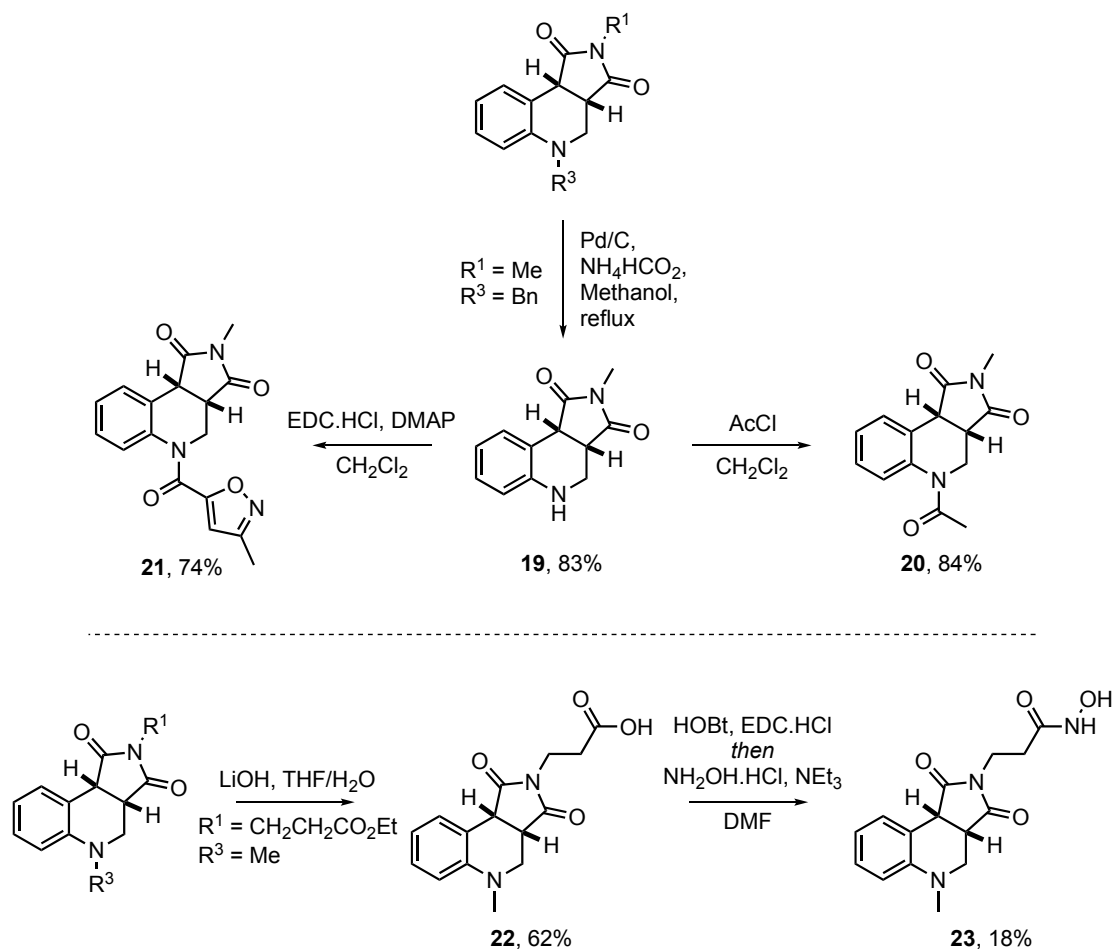
Scheme 2. Derivatizations of the tetrahydroquinoline scaffold.
