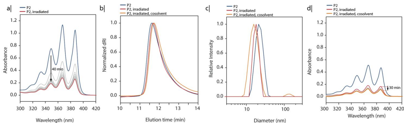
Fig. 3 a | UV-vis spectra showing the evolution of the photodimerization of anthracene in P2 in THF ( c = 1 \text{ mg}\cdot\text{mL}^{-1} ). The time on the black arrow indicates the duration of irradiation. b | Size -exclusion chromatogram of the differential refractive index (dRI) response showing the shift towards longer elution time and c | normalized distribution of sizes by DLS, respectively, of pristine P2 (blue), irradiated P2 in THF ( c = 1 \text{ mg}\cdot\text{mL}^{-1} , red), and irradiated P2 in 50/50 (v/v) THF/hexane ( c = 0.5 \text{ mg}\cdot\text{mL}^{-1} , orange) and d | UV-vis spectra showing the evolution of the photodimerization of anthracene in P2 in 50/50 (v/v) THF/hexane ( c = 0.5 \text{ mg}\cdot\text{mL}^{-1} ). The time on the black arrow indicates the duration of irradiation. Note that the blue spectrum in d | is a solution of pristine P2 in 50/50 (v/v) THF/hexane.
