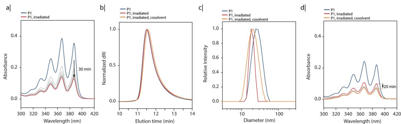
Fig. 2 a | UV-vis spectra showing the evolution of intrachain crosslinking during photodimerization of P1 in THF ( c = 1 \text{ mg}\cdot\text{mL}^{-1} ). The time on the black arrow indicates the duration of irradiation. b | Size-exclusion chromatogram of the differential refractive index (dRI) responses showing the shift towards longer elution time. c | Normalized distribution of sizes by DLS of pristine P1 (blue), irradiated P1 in THF ( c = 1 \text{ mg}\cdot\text{mL}^{-1} , red), and irradiated P1 in 50/50 (v/v) THF/hexane ( c = 0.5 \text{ mg}\cdot\text{mL}^{-1} , orange). d | UV-vis spectra showing the evolution of the photodimerization of anthracene in P1 in 50/50 (v/v) THF/hexane ( c = 0.5 \text{ mg}\cdot\text{mL}^{-1} ). The time on the black arrow indicates the duration of irradiation. Note that the blue spectrum in d | is a solution of pristine P1 in 50/50 (v/v) THF/hexane.
