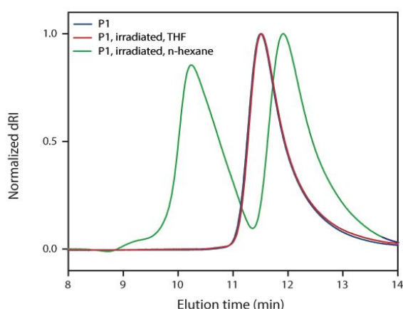
Fig. 4 Size-exclusion chromatogram of the differential refractive index (dRI) response of pristine P1 (blue), P1 irradiated in THF ( c = 1 \text{ mg}\cdot\text{mL}^{-1} , red), and P1 irradiated in pure n -hexane ( c = 1 \text{ mg}\cdot\text{mL}^{-1} , green).
