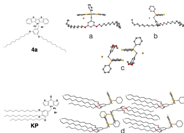
Figure 11. XRD data of phosphole-lipid ( 4a ) and phosphinine-lipid ( KP ). a), b) solid-state structures of 4a as monomers; c) the intermolecular packing of 4a (dodecyl chains are truncated for clarity); d) solid-state packing of KP . 9
