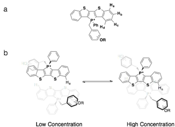
Figure 9. a) Proton assignments on the benzo moiety; b) The proposed dimerization process of phosphole-lipids. Note the position of proton H_a
