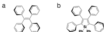
Figure 3. Examples of common AIEE chromophores. a) tetraphenylethylene; b) hexaphenylsilole
