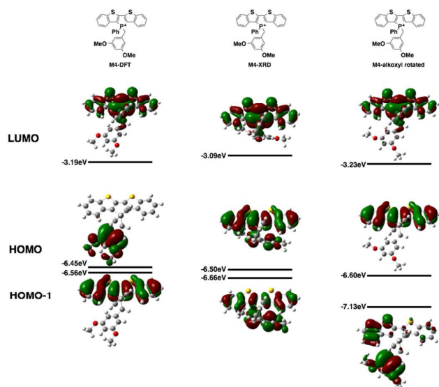
Figure 7. DFT calculations of M4 as optimized (left), based on x-ray data (middle) and M4 with the alkoxy groups rotated (right).
