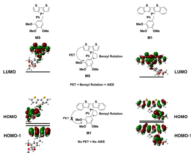
Figure 5. Mechanism of AIEE in phosphole-lipids
