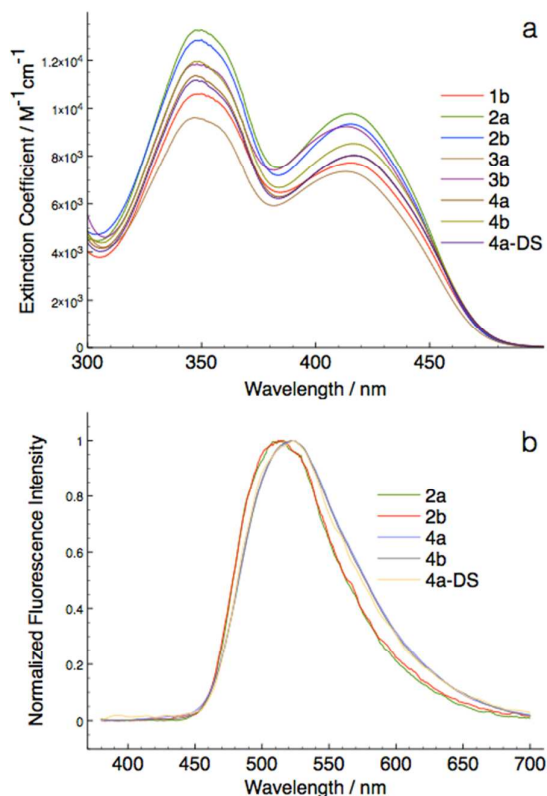
Figure 4. Solution photophysics of phosphole-lipids. a) UV-Vis absorption spectra of the phosphole-lipids; b) Fluorescence spectra of phosphole-lipids (low emission species was omitted for clarity due to low signal to noise ratio).
