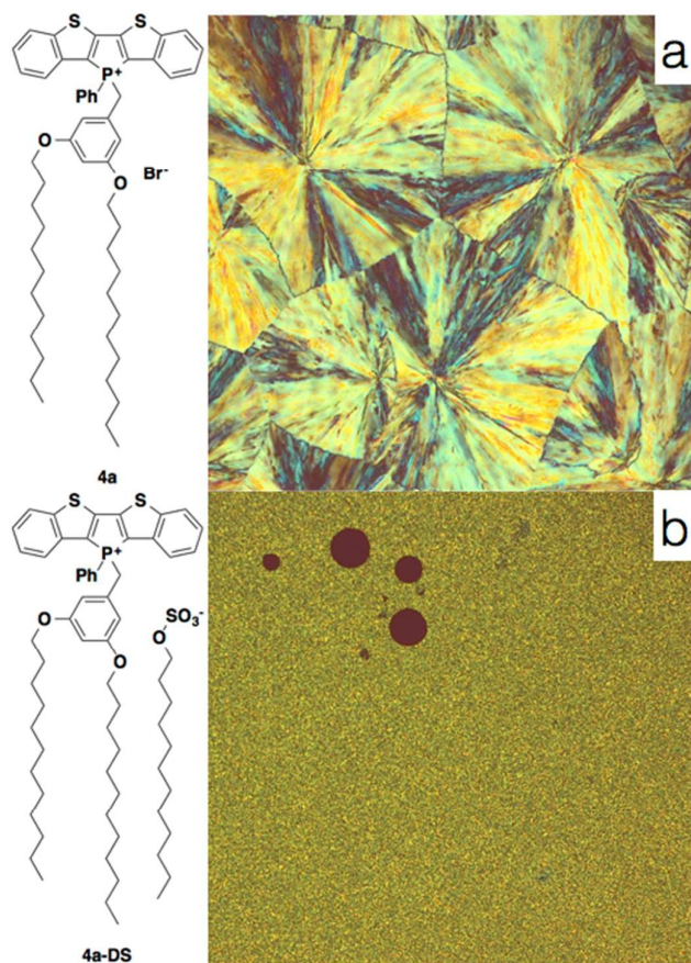
Figure 14. Polarized optical microscopy of 4a (a) and 4a-DS (b). Note the differences in domain size between the two micrograph
