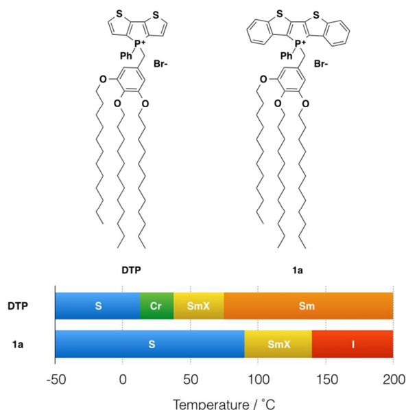
Figure 2. Phosphole-lipid liquid crystals. S, "solid"; Cr, crystalline state; SmX, soft crystal; Sm, smectic phase; I, isotropic liquid
