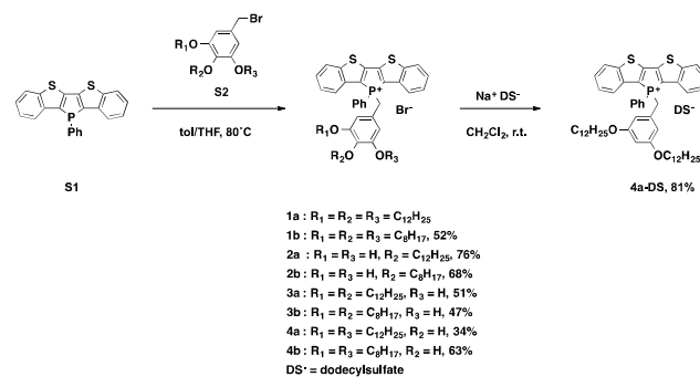
Scheme 1. Synthesis of phosphole-lipids. Quaternization of S1 with various benzyl bromides ( S2 ) afforded the desired phosphole-lipids 1-4 . The bromide anion was exchanged with dodecylsulfate via metathesis.
