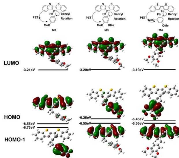
Figure 6. Frontier orbitals of model phosphole-lipids
