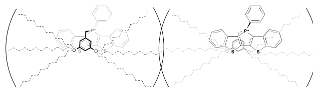
Figure 12. Proposed mechanism for intermolecular repulsion of 4a in solution
