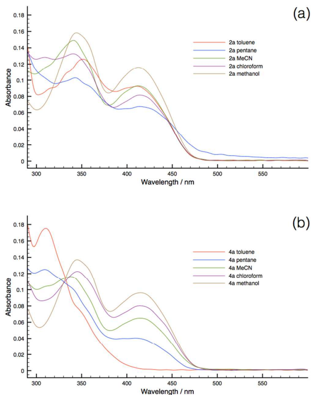
Figure 8. Solvatochromism of 2a (top) and 4a (bottom). All experiments were conducted at 10^{-5} M to mitigate effect of aggregation. a) Absorption of 2a in various solvents; b) Absorption of 4a in various solvents, note the disappearance of the high-energy band at 300nm and the appearance of the low energy bands at 350 nm and 420 nm, respectively.
