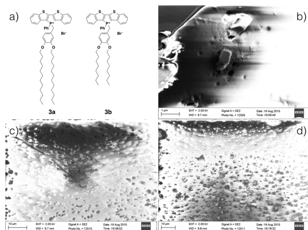
Figure 10. Scanning electron microscopy of 3 series of phosphole-lipids. a) phosphole-lipids 3a and 3b ; b) crystallites on the surface of 3b film; c) amorphous surface of 3a film; d) amorphous surface of 3b film with crystallites on the surface.
