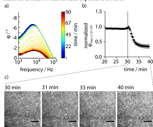
Fig. 4. Monitoring of epithelial barrier disruption by ionomycin using the transparent conductive polymer-based 2-electrode PAS sensor. (a) Partial PAS spectra of cells exposed to ionomycin after 30 min baseline recording. Spectra were achieved at 10^3 - 10^5 Hz with 30 s time resolution. The colour-coded time parameter shows decay of epithelial integrity by the decreased amplitude of the peak \phi values. (b) Extracted, normalized \phi peak values show the kinetics of epithelial barrier degeneration. (mean \pm SEM, n = 3 ) (c) Phase contrast microscopy performed simultaneously to PAS sensing. (20X, scale bar = 200 \mu m).
