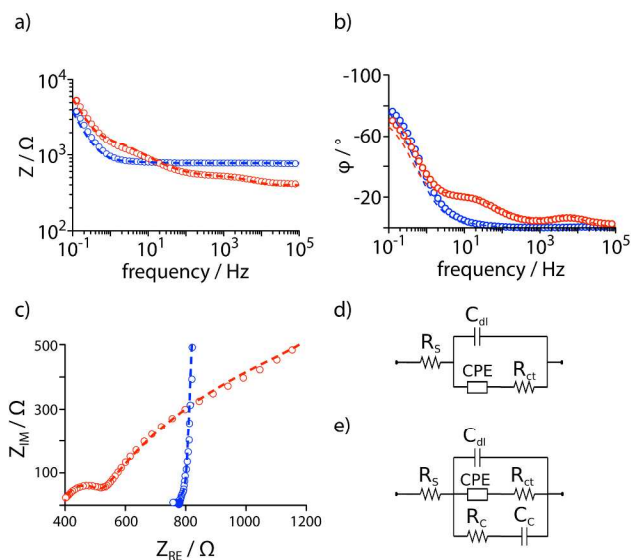
Fig. 2. EIS of electrodeposited PEDOT:PSS in the absence (blue) and presence (red) of a confluent layer of MDCK cells in supplemented cell culture medium. (a) Impedance Z and (b) phase angle \phi presented in Bode plots. (c) A Nyquist plot shows Z_{RE} and Z_{IM} as polar coordinates, Z(\omega) = Z_{IM} \sin \phi^{-1} = Z_{RE} \cos \phi^{-1} , \omega = 2\pi f . Data were fitted with an equivalent circuit model adapted from Richardson-Burns et al. 12 Experimental data = open circles, fitted data = dashed lines. (d) The equivalent circuit used to fit EIS data in supplemented cell culture medium only. (e) The extended equivalent circuit model used to fit EIS data arising from a confluent monolayer of cells on the PEDOT:PSS PAS electrodes.
