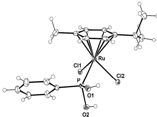
Fig. 2 ORTEP-diagram of 6^{\text{OH}} with 30% probability ellipsoids. Hydrogen atoms, except for O(1) and O(2), are omitted for clarity. Selected bond length (Å) and angles (°): Ru(1)-P(1), 2.2969(9); Ru(1)-Cl(1), 2.4245(8); Ru(1)-Cl(2), 2.4275(9); Ru(1)-centroid(Cp), 1.7045; P(1)-Ru(1)-Cl(1), 87.27(3); P(1)-Ru(1)-Cl(2), 82.78(3).
