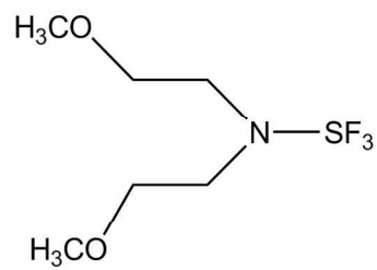
Deoxo-Fluor
