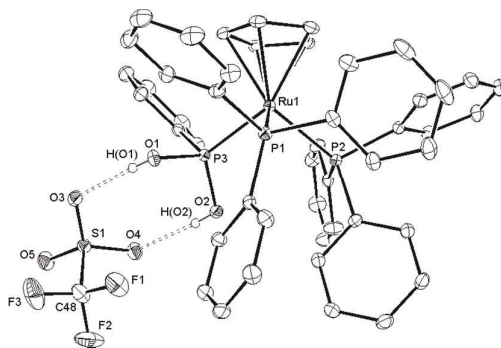
Fig. 1. ORTEP-diagram of 3 OH CCl 2 with 30% probability ellipsoids. Hydrogen atoms, except for O(1) and O(2) are omitted for clarity. Selected bond length (Å) and angles (°): Ru(1)-P(1), 2.3670(7); Ru(1)-P(2), 2.3408(7); Ru(1)-P(3), 2.2745(7); Ru-centroid(Cp), 1.8959; O(3)-H(O1), 2.0401; O(4)-H(O2), 2.0177; P(1)-Ru(1)-P(2), 98.20(2); P(1)-Ru(1)-P(3), 97.74(2); P(2)-Ru(1)-P(3), 96.37(2).
