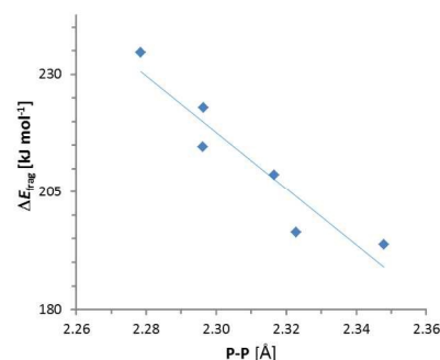
Fig. 5: Plot of computed fragmentation energies ΔE frag vs. bond distances. The straight line is the result of a linear regression analysis (R 2 = 0.89).
