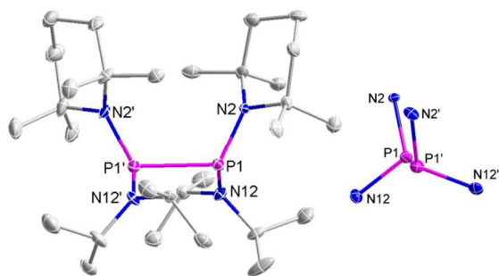
Figure 1: Representation of the molecular structure of \{9\}_2 in the crystal (left) and reduced plot of the central P_2N_4 skeleton (right). Thermal ellipsoids were drawn at 50% probability level, and H atoms were omitted for clarity. Selected bond lengths [Å]: P1-N12 1.727(5), P1-N2 1.738(5), P1-P1' 2.357(2), P1'-N12' 1.711(5), P1'-N2' 1.740(5).
