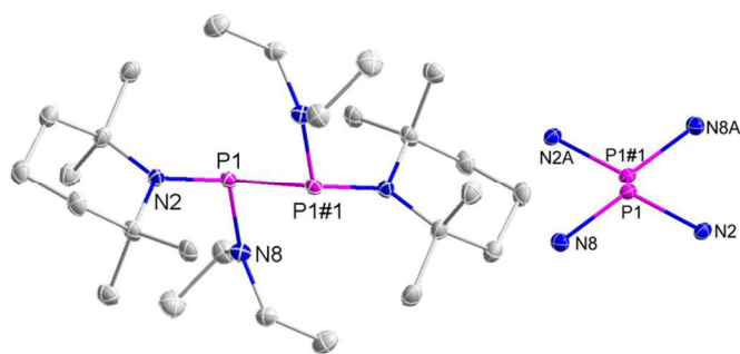
Figure 1: Representation of the molecular structure of \{8\}_2 in the crystal (left) and reduced plot of the central P_2N_4 skeleton (right). Thermal ellipsoids were drawn at 50% probability level, and H atoms were omitted for clarity. Selected bond lengths [Å]: P1-N8 1.7070(16), P1-N2 1.7395(15), P1-P1#1 2.2914(10).
