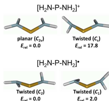
Fig. 6: Computed molecular structures and relative energies (in \text{kJ mol}^{-1} ) at the CCSD/aug-cc-pVDZ level of theory for the electronic ground states (left) and rotational transition states (right) of 10'' and 10' .
