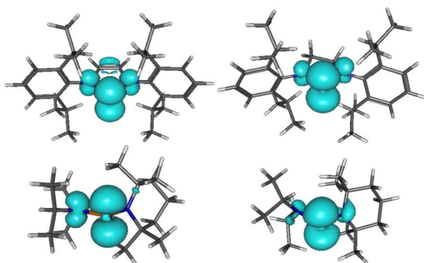
Figure 3: Representation of computed ( \omega B97x-D/cc-pVDZ) spin densities in the radicals 3c (top left), 4 (top right), 9 (bottom left), and a second conformer of 9 with skewed alignment of R 2 N-groups (bottom right; skew angles 69° and 59°). The two conformers of 9 illustrate the dependence of N-centred spin density on skew angles. The drawn isodensity surfaces include 75% of the total spin density.
