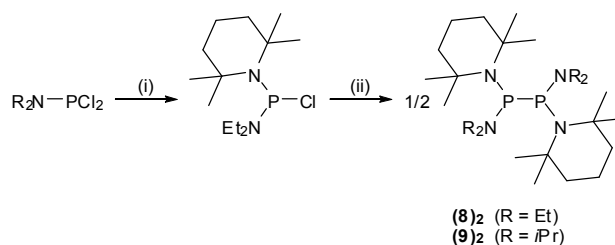
Scheme 3: Synthesis of the diphosphanes {8} 2 , {9} 2 . Reaction conditions: (i) 1 equiv. Li(tetramethylpiperidyl), THF, –78 °C to r.t.; (ii) excess Mg in THF ( {8} 2 ) or Na in hexane ( {9} 2 ), 3 – 7 h ultrasound at 48 °C.
