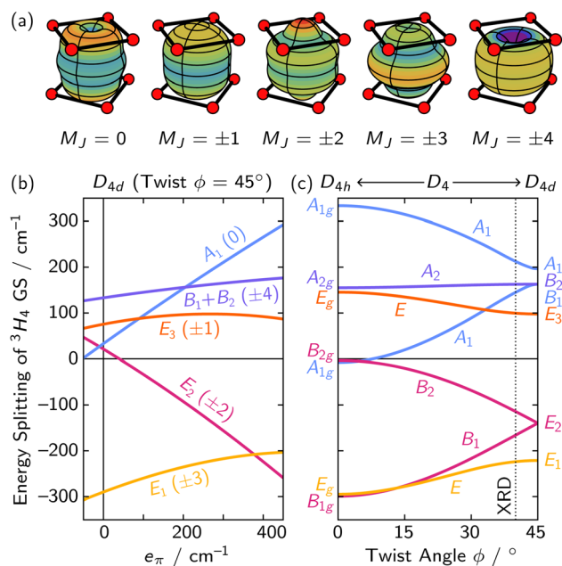
Fig. 3 (a) Charge density distributions for the M_J levels within the ^3H_4 GS of Pr^{III} show the \pm 3 levels should be lowest in energy. (b) The predicted splitting from an AOM treatment of 1\cdot Pr in perfect D_{4d} symmetry using e_\sigma = 400\text{ cm}^{-1} . (c) Deviations from ideal D_{4d} symmetry ( 45^\circ twist) cause descent into D_4 symmetry. Notably, this splits the E_2 level into a B_1 and a B_2 level ( e_\sigma = 400\text{ cm}^{-1} , e_\pi = 265\text{ cm}^{-1} ).
