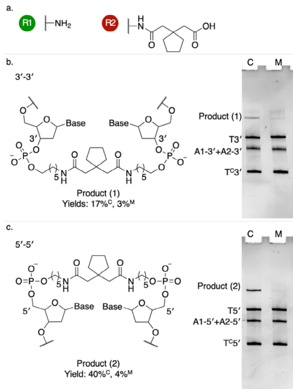
Fig. 2 DNA-templated amide bond formation. (a) Reactive building blocks. (b) Product of reaction across 3'–3' and (c) 5'–5' ends (SI Methods). Strands T C , A1–NH 2 and A2–COOH were annealed in MOPS buffer (pH 7.7) supplemented with MgCl 2 . After annealing then equilibration at 24 °C for 20 h, DMT–MM was added to activate amide coupling (final concentrations: 91 nM T C , 99 nM A1–NH 2 , 99 nM A2–COOH, 23 mM MOPS buffer, 18 mM MgCl 2 , 45 mM DMT–MM in a total volume of 35.2 μL). The reaction was run at 25 °C for 20 h. Lane C: fully complementary triplex sequences. Lane M: templating duplex mutated to disrupt triplex formation.
