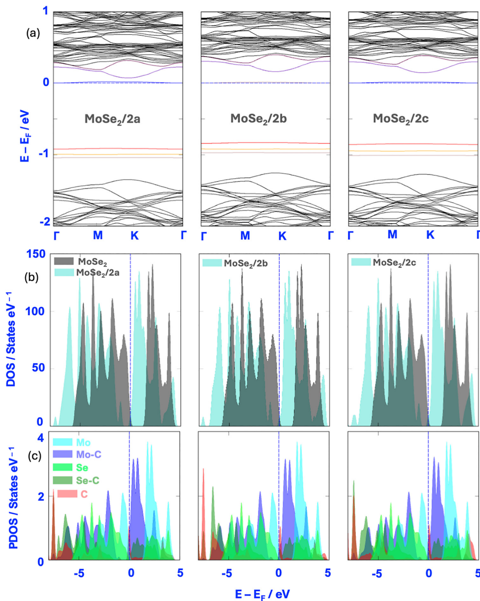
Fig. 2 The band structure (a), DOS (b), and PDOS (c) plots for MoSe 2 /2a, MoSe 2 /2b, and MoSe 2 /2c show the bandgap and Fermi level for each material. The PDOS for each element is indicated by the color legend.
