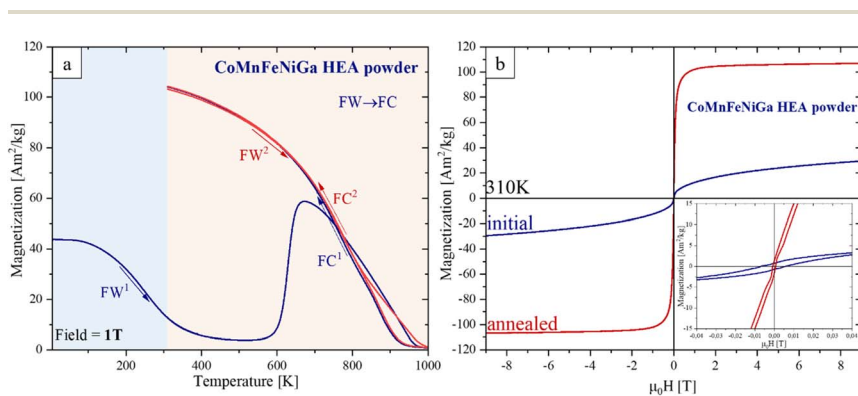
Fig. 8 CoMnFeNiGa HEA micropowder: (a) temperature-dependent magnetization M(T) recorded at 1 T, (b) field-dependent magnetization M(H) measured at 310 K before and after annealing ( -9\text{ T} \geq B_{\text{ext}} \geq 9\text{ T} ).
