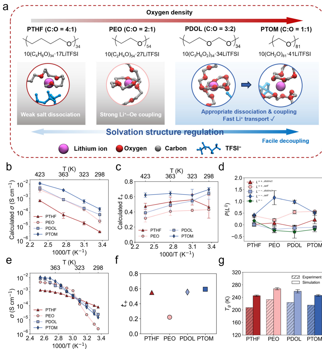
Fig. 1 Effects of oxygen density on transport properties of ether-based polymer electrolytes. (a) Schematic illustration of ether-based polymers in SPEs systems, solvation structures, and the effect on Li + transport in the contribution. The variation in oxygen density along the polymer backbone influences the Li + solvation structure, tuning the Li + –Oe binding strength and results in optimal Li + transport. Hydrogen atoms are omitted in the snapshot of the solvation structure for clarity. The calculated (b) ionic conductivity ( \sigma ), (c) Li + transference number ( t_+ ) from MD simulations, and (d) Onsager transport coefficient analysis. The experimental measured (e) \sigma and (f) t_+ . (g) The measured and calculated T_g .
