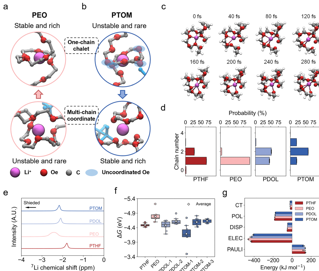
Fig. 3 Structural origins of the transport mode transitions. Representative Li + solvation structure in (a) PEO and (b) PTOM. Hydrogen atoms are omitted for clarity. The one-chain chelate of PEO displays continuous coordination, whereas that of PTOM exhibits discontinuous coordination. In PEO, the one-chain chelate is more stable than the multi-chain coordinate complex, while it is the opposite in PTOM. (c) The discontinuous coordination (DC) structure observed in the AIMD simulation of PTOM. The uncoordinated oxygen and the coordinated oxygen swap frequently. (d) The statistical binding polymer chain number of Li + . (e) Solid-state 7 Li NMR spectra, (f) binding free energy of the representative Li + -polymer complex; the numbers represent the binding chain number of Li + , and (g) binding energy decomposition into contributions of permanent electrostatics (ELEC), Pauli repulsion (PAULI), dispersion (DISP), polarization (POL), and charge transfer (CT) for different systems.
