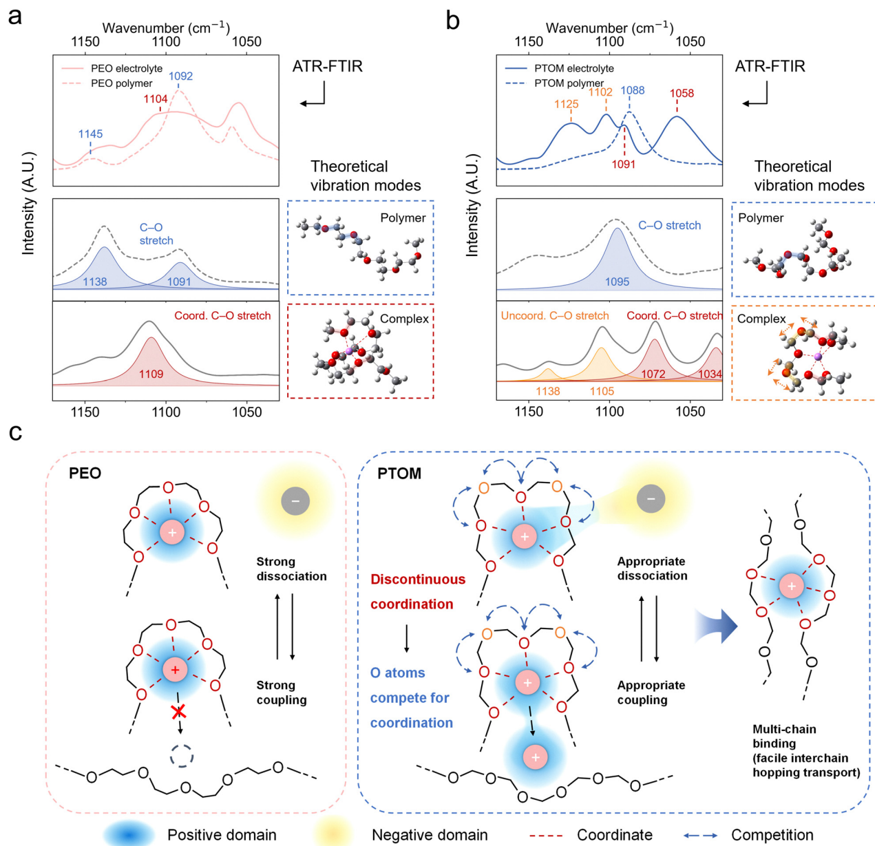
Fig. 4 The identification of the discontinuous coordination structure and its effect on \text{Li}^+ transport behavior. The ATR-FTIR spectra of (a) PEO electrolyte and PEO polymer, as well as (b) PTOM electrolyte and PTOM polymer. The first row presents the experimental results, and the second and third rows display the theoretically calculated vibration modes and the corresponding structures. (c) Schematic illustration of the mechanism of the solvation structure affecting the \text{Li}^+ transport in PEO and PTOM.
