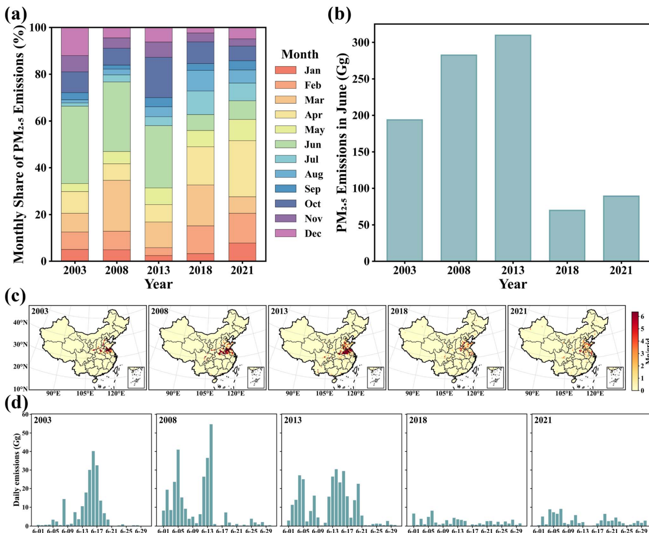
Fig. 1 OCSB \text{PM}_{2.5} emissions over China in 2003, 2008, 2013, 2018, and 2021. (a) Monthly shares of annual \text{PM}_{2.5} emissions from OCSB. (b) Nation-wide total emissions in June. (c) Mean spatial distribution of \text{PM}_{2.5} emissions in June. (d) Nation-wide daily total \text{PM}_{2.5} emissions in June.
