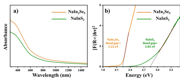
Figure 4: Optical property analysis a) Absorbance spectrum b) Tauc plot analysis for for \text{NaIn}_3\text{Se}_5 and \text{NaInS}_2 NCs
